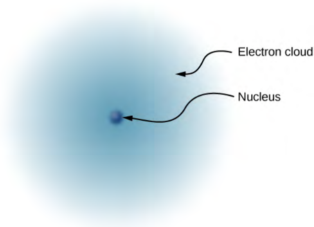
Figure 5.7 This simplified model of a hydrogen atom shows a positively charged nucleus (consisting, in the case of hydrogen, of a single proton), surrounded by an electron “cloud.” The charge of the electron cloud is equal (and opposite in sign) to the charge of the nucleus, but the electron does not have a definite location in space; hence, its representation here is as a cloud. Normal macroscopic amounts of matter contain immense numbers of atoms and molecules, and, hence, even greater numbers of individual negative and positive charges.
