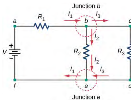
Figure 10.24 At first glance, this circuit contains two junctions, Junction b and Junction e , but only one should be considered because their junction equations are equivalent.
