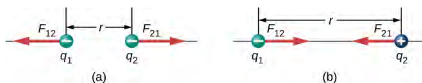
Figure 5.14 The electrostatic force \vec{\mathbf{F}} between point charges q_1 and q_2 separated by a distance r is given by Coulomb's law. Note that Newton's third law (every force exerted creates an equal and opposite force) applies as usual—the force on q_1 is equal in magnitude and opposite in direction to the force it exerts on q_2 . (a) Like charges; (b) unlike charges.
