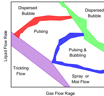
Fig. -13.7. A dimensional vertical flow map under very low gravity against the gravity.
