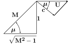
Fig. -12.22. The angles of the Mach line triangle.
