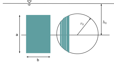
Fig. -4.34. Schematic of Immersed Cylinder.
