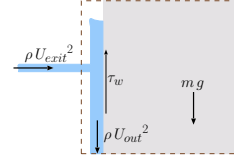
Fig. -6.12. Jet impinging jet surface perpendicular and with the surface.
