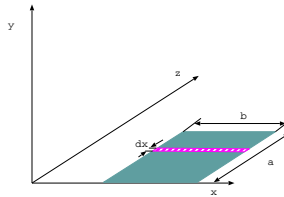
Fig. -3.7. Description of rectangular in x - z plane for calculation of moment of inertia.
