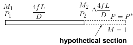
Fig. -11.33. Unchoked flow calculations showing the hypothetical "full" tube when choked
