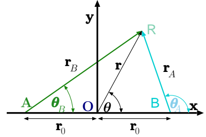
Fig. -10.10. Combination of the Source and Sink located at a distance r_0 from the origin on the x coordinate. The source is on the right.
