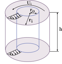
Fig. -1.13. Concentrating cylinders with the rotating inner cylinder.
