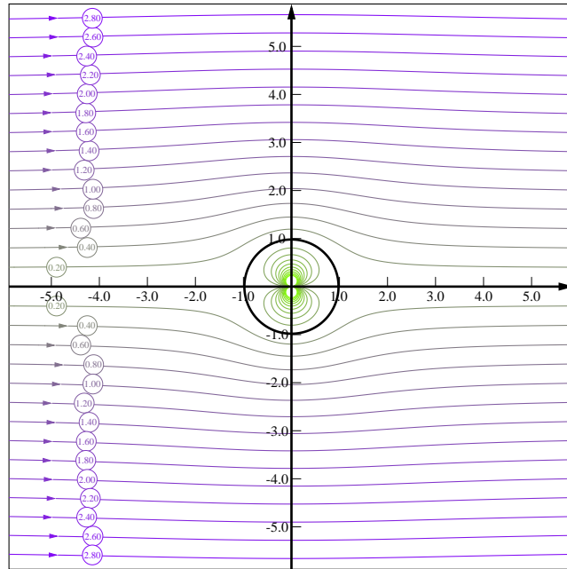
Fig. -10.13. Stream function of uniform flow plus doublet results in solid body with flow around it. Stream function ( \psi and not \psi ) starts from -2.0 (green line) to 3 the (purple line). The negative streamlines lines are inside the solid body. The arrows are calculated by trapping the y for given \psi around the end points. Hence, the slight difference between the arrow and the line. The more negative the stream function the smaller the counter. The larger positive stream function the further away the line form the x coordinate. It can be noticed closer the "solid body" the lines are more curved. The GLE code is attached in the source code to this book. The value of n is the bubbles.
