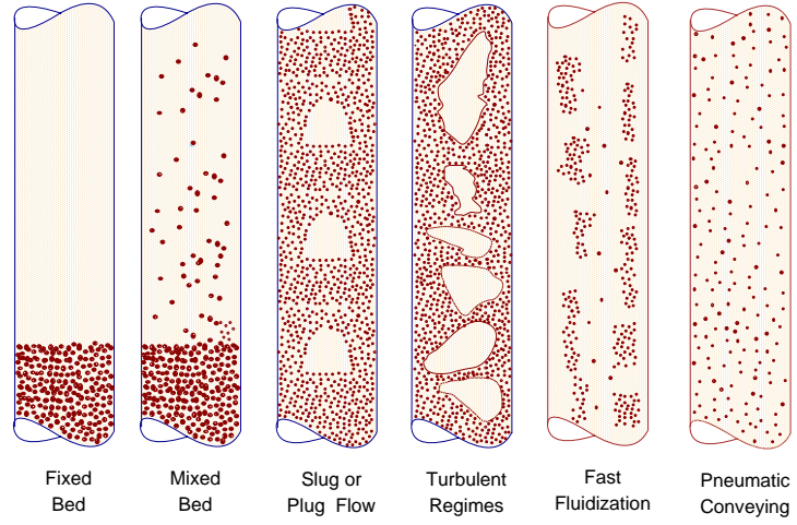
Fig. -13.9. The flow patterns in solid-liquid flow.
