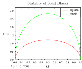
Fig. -4.42. The maximum height reverse as a function of density ratio.
