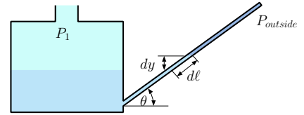
Fig. -4.8. Inclined manometer.
