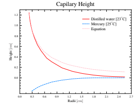
Fig. -1.25. The raising height as a function of the radius.
