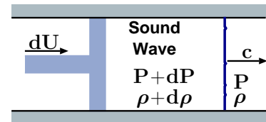
Fig. -11.1. A very slow moving piston in a still gas.
