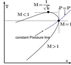
Fig. -11.38. The temperature entropy diagram for Rayleigh line.
