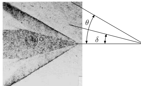
Fig. -12.11. Oblique shock occurs around a cone. This photo is courtesy of Dr. Grigory Toker, a Research Professor at Cuernavaca University of Mexico. According to his measurement, the cone half angle is 15^\circ and the Mach number is 2.2.
