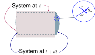
Fig. -7.1. The work on the control volume is done by two different mechanisms, S_n and \tau .
