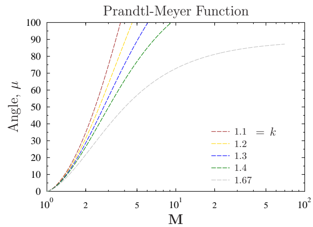
Fig. -12.26. The angle as a function of the Mach number and spesfic heat.
