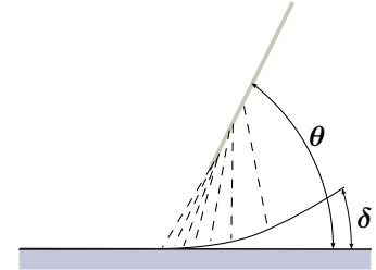
Fig. -12.10. A local and a far view of the oblique shock.
