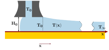
Fig. -8.4. Mass flow in coating process for example 8.2.
