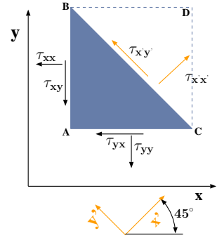
Fig. -8.10. Shear stress at two coordinates in 45° orientations.
