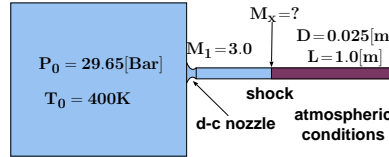
Fig. -11.22. The schematic of Example (11.19).
