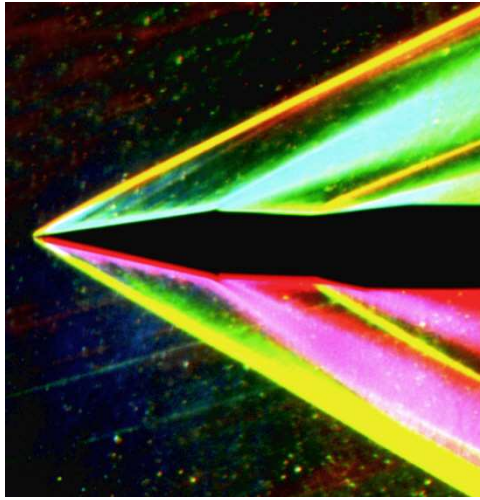
Fig. -12.9. Color-schlieren image of a two dimensional flow over a wedge. The total deflection angel (two sides) is 20^\circ and upper and lower Mach angel are \sim 28^\circ and \sim 30^\circ , respectively. The image show the end-effects as it has thick (not sharp transition) compare to shock over a cone. The image was taken by Dr. Gary Settles at Gas Dynamics laboratory, Penn State University.
