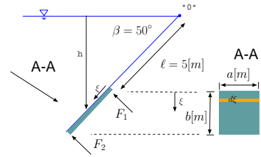
Fig. -4.20. Rectangular area under pressure.
