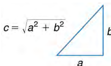
Figure 3.4 The Pythagorean theorem relates the length of the legs of a right triangle, labeled a and b , with the hypotenuse, labeled c . The relationship is given by: a^2 + b^2 = c^2 . This can be rewritten, solving for c : c = \sqrt{a^2 + b^2} .
