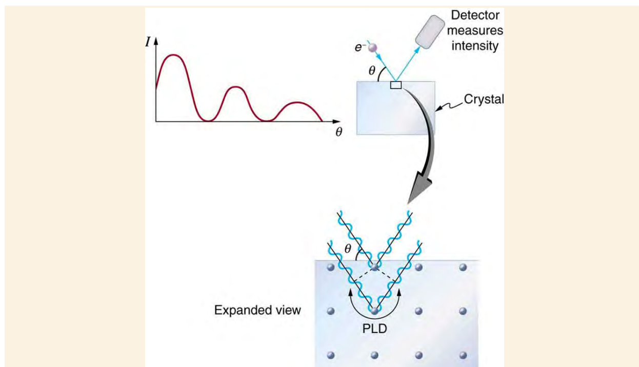
Figure 29.24 The diffraction pattern at top left is produced by scattering electrons from a crystal and is graphed as a function of incident angle relative to the regular array of atoms in a crystal, as shown at bottom. Electrons scattering from the second layer of atoms travel farther than those scattered from the top layer. If the path length difference (PLD) is an integral wavelength, there is constructive interference.
