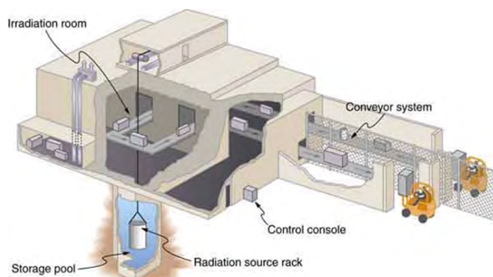
Figure 32.14 A food irradiation plant has a conveyor system to pass items through an intense radiation field behind thick shielding walls. The \gamma source is lowered into a deep pool of water for safe storage when not in use. Exposure times of up to an hour expose food to doses up to 10^4 Gy.
