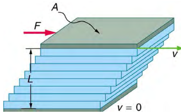
Figure 12.12 The graphic shows laminar flow of fluid between two plates of area A . The bottom plate is fixed. When the top plate is pushed to the right, it drags the fluid along with it.
