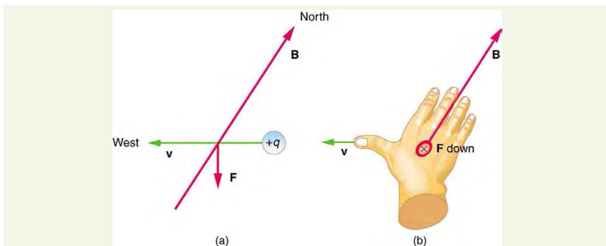
Figure 22.18 A positively charged object moving due west in a region where the Earth's magnetic field is due north experiences a force that is straight down as shown. A negative charge moving in the same direction would feel a force straight up.
