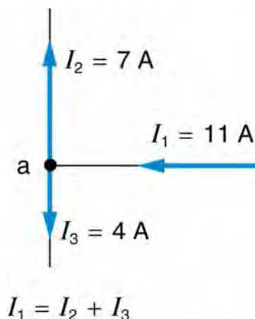
Figure 21.22 The junction rule. The diagram shows an example of Kirchhoff's first rule where the sum of the currents into a junction equals the sum of the currents out of a junction. In this case, the current going into the junction splits and comes out as two currents, so that I_1 = I_2 + I_3 . Here I_1 must be 11 A, since I_2 is 7 A and I_3 is 4 A.
