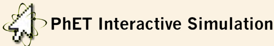
Figure 31.29 Nuclear Fission ( http://cnx.org/content/m42640/1.5/nuclear-fission_en.jar )
