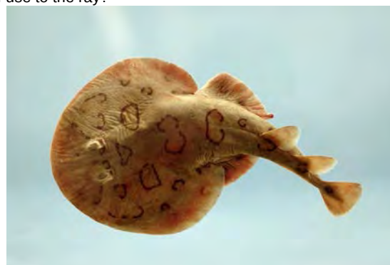
Figure 19.32 Lesser electric ray ( Narcine bancroftii ) (credit: National Oceanic and Atmospheric Administration, NOAA's Fisheries Collection).
