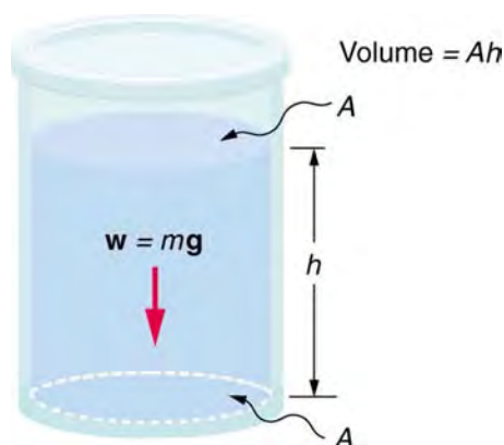
Figure 11.10 The bottom of this container supports the entire weight of the fluid in it. The vertical sides cannot exert an upward force on the fluid (since it cannot withstand a shearing force), and so the bottom must support it all.
