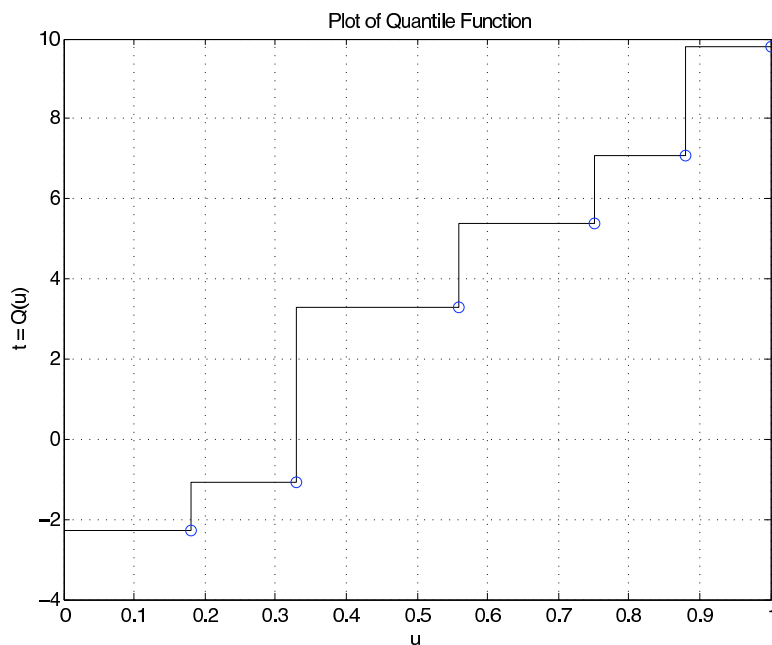
Figure 10.57: Quantile function for Example 10.32 (Simple Random Variable).
