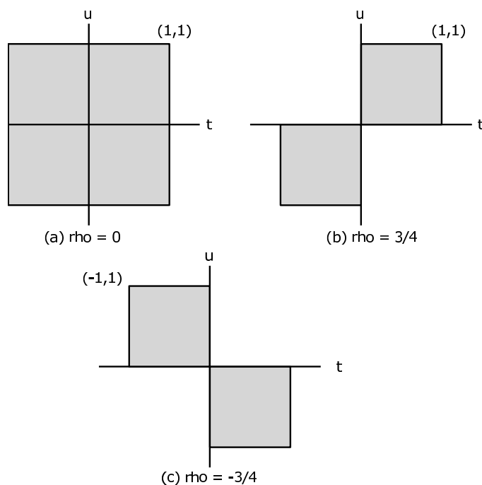
Figure 12.63: Uniform marginals but different correlation coefficients.
