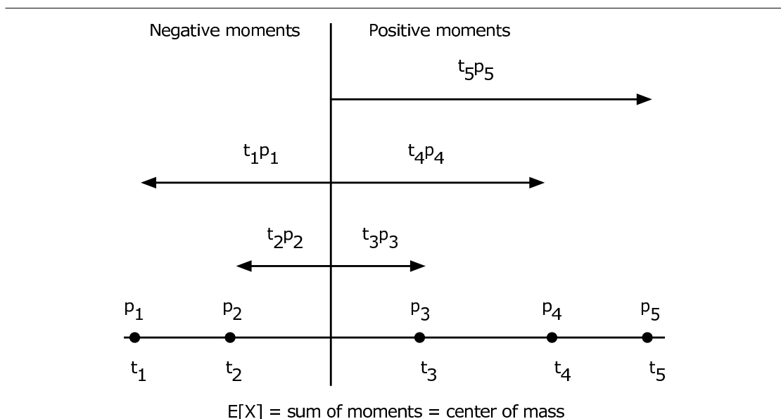
Figure 11.5: Moment of a probability distribution about the origin.
