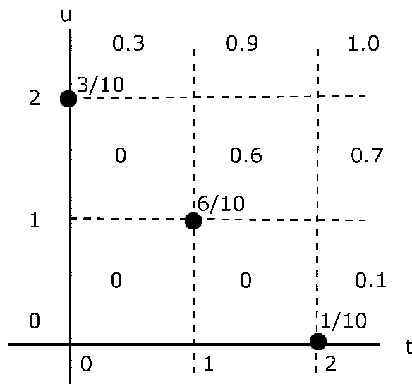
Figure 8.6: The joint distribution for Example 8.3 (Distribution function for the selection problem in Example 8.1 (A selection problem)).
