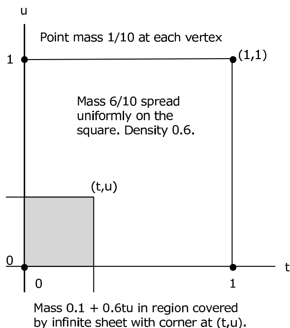
Figure 8.9: Mixed joint distribution for Example 8.4 (A mixed distribution).
