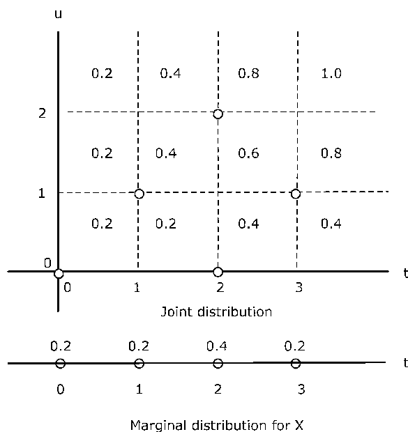
Figure 8.13: Marginal distribution for Example 1.
