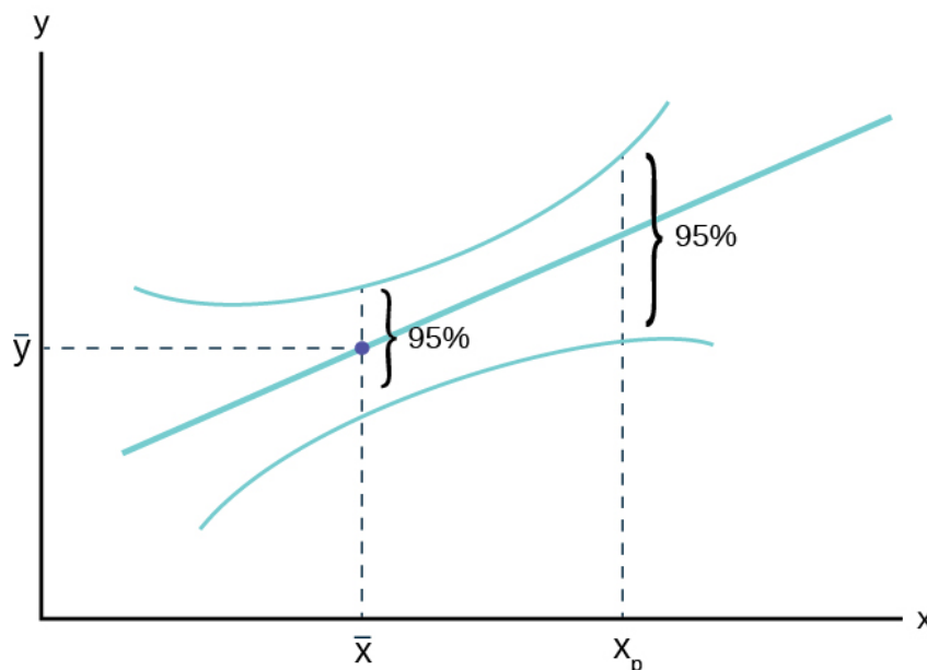
Figure 13.15 Confidence interval for an individual value of x , X_p , at 95% level of confidence
