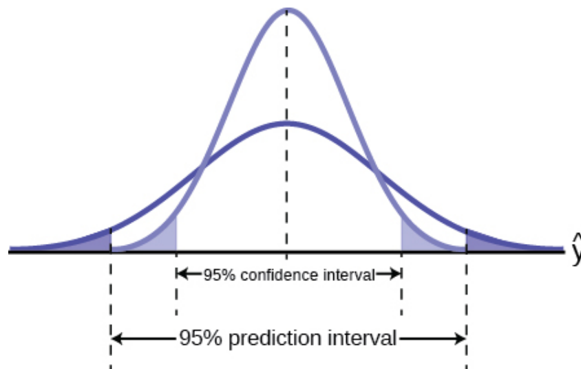
Figure 13.14 Prediction and confidence intervals for regression equation; 95% confidence level.
