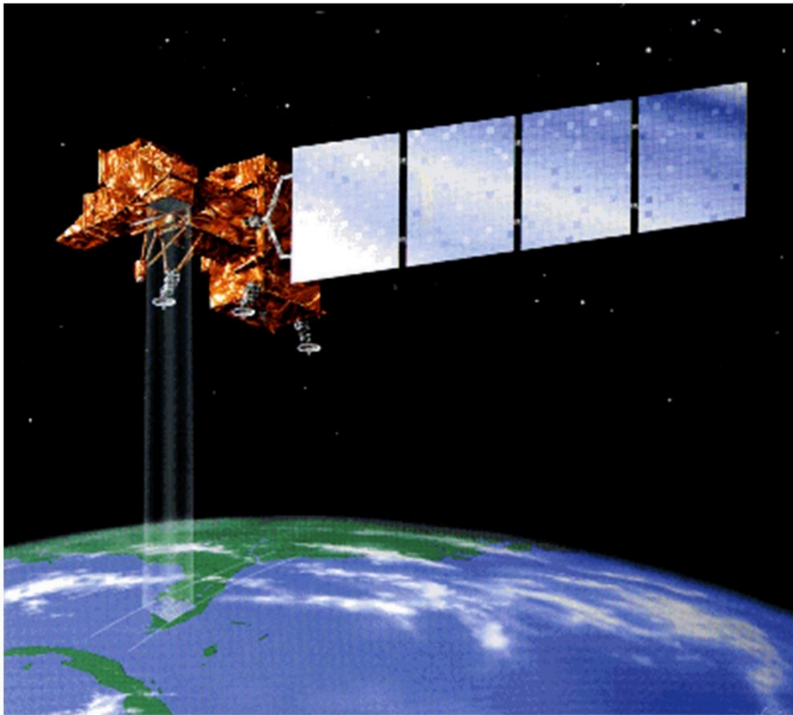
Satellite imaging. Painting of the Landsat 7 remote sensing satellite. Note that the satellite does not really cast a four-sided beam of light upon the Earth's surface, this is just artistic licence. Instead, the satellite's sensors record electromagnetic energy reflected or emitted by the Earth. 8
