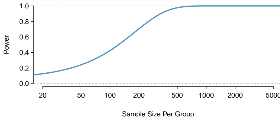
Figure 5.20: The curve shows the power for different sample sizes in the context of the blood pressure example when the true difference is -3. Having more than about 250 to 350 observations doesn't provide much additional value in detecting an effect when \alpha = 0.05 .
