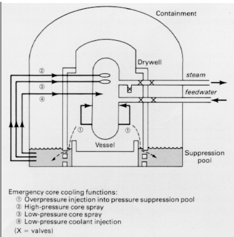
Figure 6. BWR emergency core cooling systems
