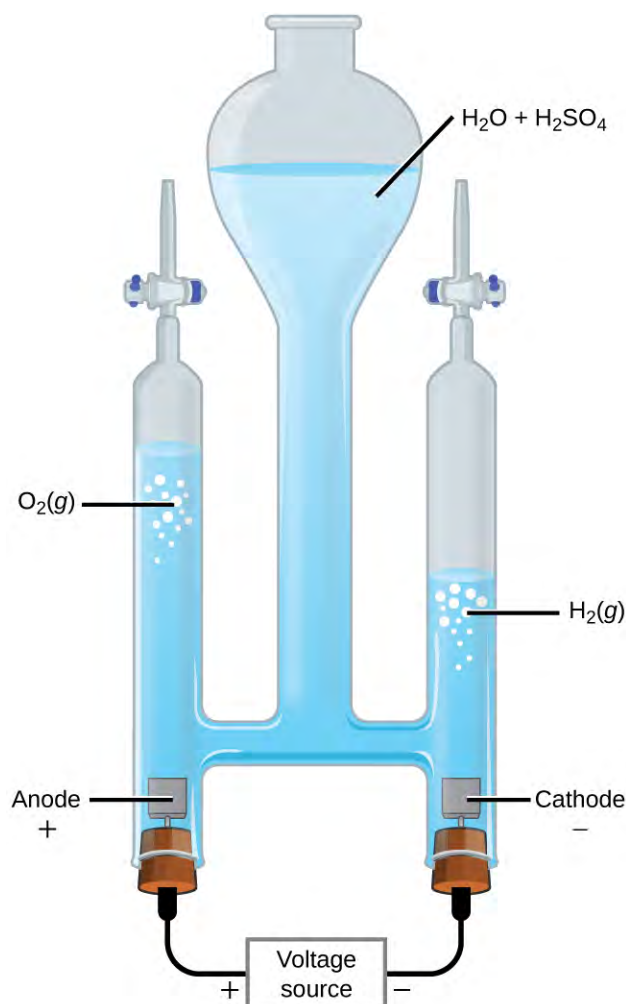
Figure 17.20 Water decomposes into oxygen and hydrogen gas during electrolysis. Sulfuric acid was added to increase the concentration of hydrogen ions and the total number of ions in solution, but does not take part in the reaction. The volume of hydrogen gas collected is twice the volume of oxygen gas collected, due to the stoichiometry of the reaction.
