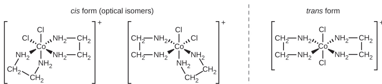
Figure 19.24 Three isomeric forms of [Co(en)_2Cl_2]^+ exist. The trans isomer, formed when the chlorines are positioned at a 180^\circ angle, has very different properties from the cis isomers. The mirror images of the cis isomer form a pair of optical isomers, which have identical behavior except when reacting with other enantiomers.
