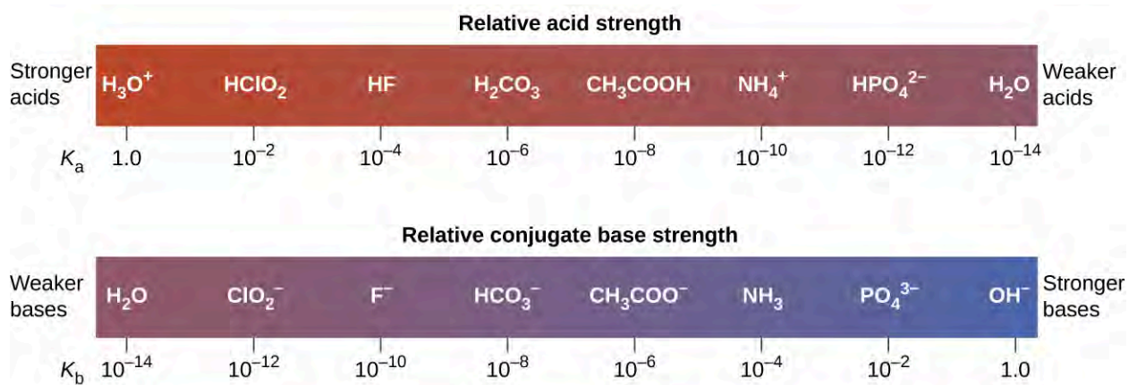
Figure 14.7 This diagram shows the relative strengths of conjugate acid-base pairs, as indicated by their ionization constants in aqueous solution.
