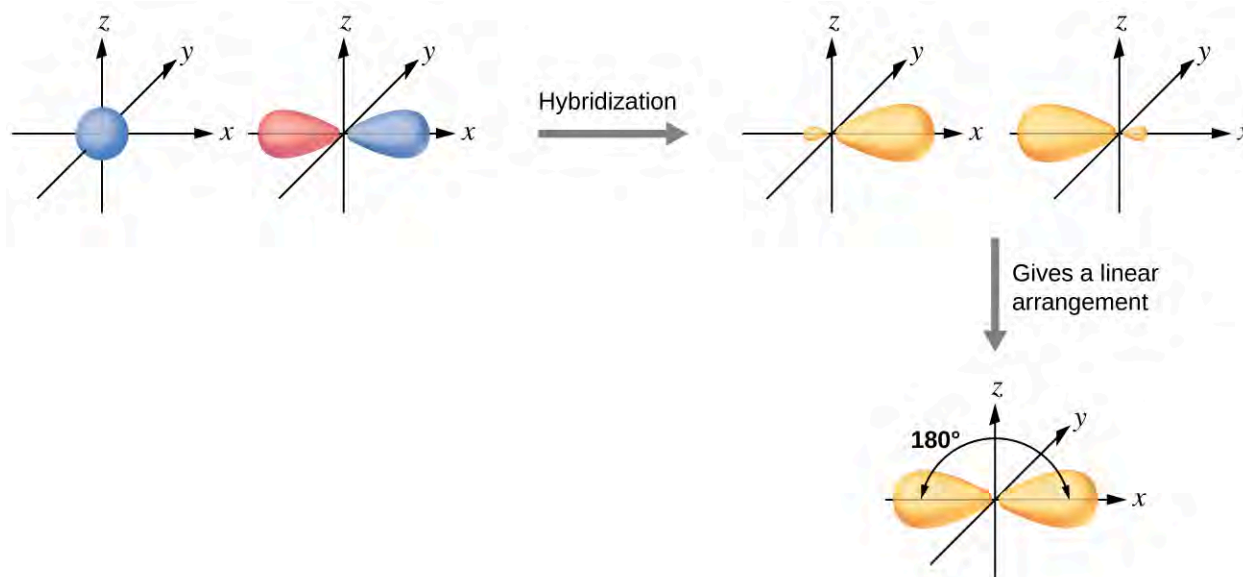
Figure 8.8 Hybridization of an s orbital (blue) and a p orbital (red) of the same atom produces two sp hybrid orbitals (yellow). Each hybrid orbital is oriented primarily in just one direction. Note that each sp orbital contains one lobe that is significantly larger than the other. The set of two sp orbitals are oriented at 180^\circ , which is consistent with the geometry for two domains.
