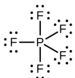
Trigonal bipyramid
