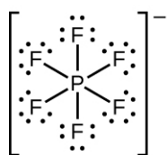
Octahedral
