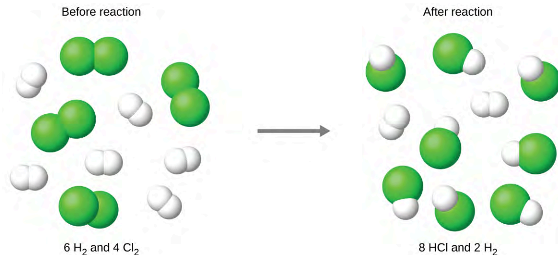
Figure 4.13 When \text{H}_2 and \text{Cl}_2 are combined in nonstoichiometric amounts, one of these reactants will limit the amount of \text{HCl} that can be produced. This illustration shows a reaction in which hydrogen is present in excess and chlorine is the limiting reactant.
