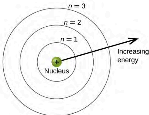
Figure 6.20 Different shells are numbered by principal quantum numbers.
