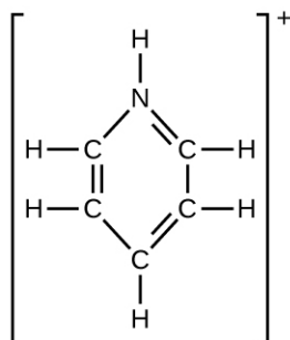
pyridinium ion, trigonal planar, sp^2
