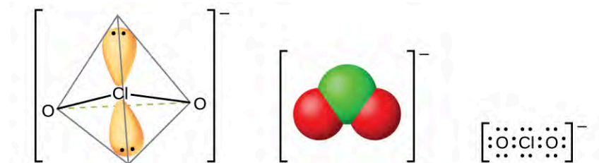
Figure 18.55 Chlorite ions, \text{ClO}_2^- , are produced when chlorous acid reacts with bases.
