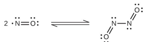
Figure 18.34 This shows the equilibrium between NO and N 2 O 2 . The molecule, N 2 O 2 , absorbs light.
