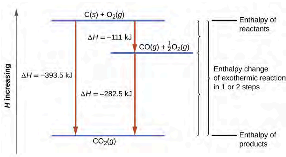
Figure 5.24 The formation of \text{CO}_2(\text{g}) from its elements can be thought of as occurring in two steps, which sum to the overall reaction, as described by Hess's law. The horizontal blue lines represent enthalpies. For an exothermic process, the products are at lower enthalpy than are the reactants.
