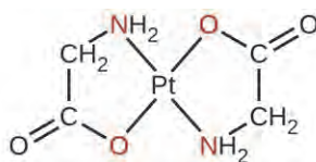
Figure 19.17 Each of the anionic ligands shown attaches in a bidentate fashion to platinum(II), with both a nitrogen and oxygen atom coordinating to the metal.
