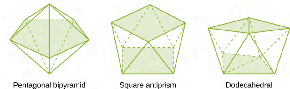
Figure 19.18 These are geometries of some complexes with coordination numbers of seven and eight.
