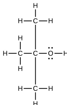
Compound C
