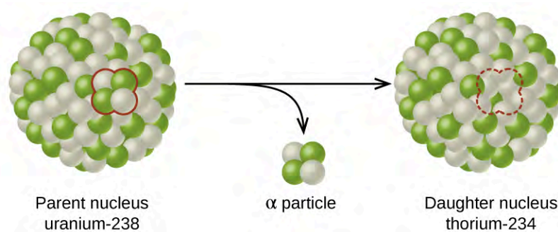
Figure 21.5 A nucleus of uranium-238 (the parent nuclide) undergoes \alpha decay to form thorium-234 (the daughter nuclide). The alpha particle removes two protons (green) and two neutrons (gray) from the uranium-238 nucleus.
