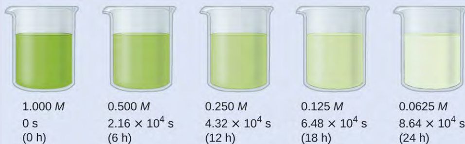
Figure 12.13 The decomposition of H 2 O 2 (2H 2 O 2 → 2H 2 O + O 2 ) at 40 °C is illustrated. The intensity of the color symbolizes the concentration of H 2 O 2 at the indicated times; H 2 O 2 is actually colorless.
