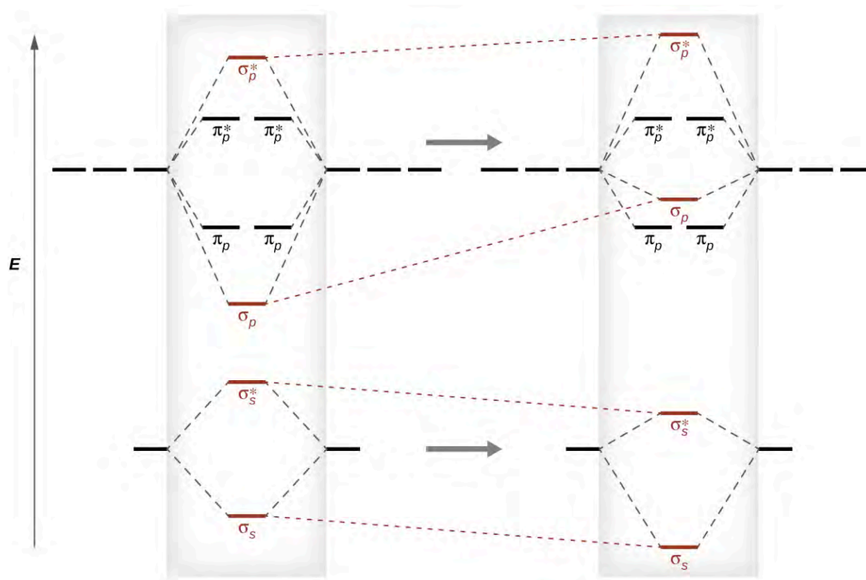
Figure 8.38 Without mixing, the MO pattern occurs as expected, with the \sigma_p orbital lower in energy than the \pi_p orbitals. When s-p mixing occurs, the orbitals shift as shown, with the \sigma_p orbital higher in energy than the \pi_p orbitals.
