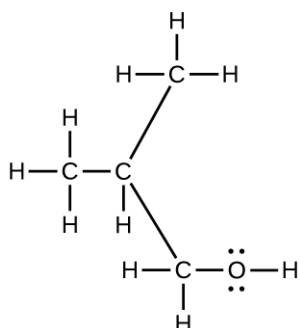
Compound A
