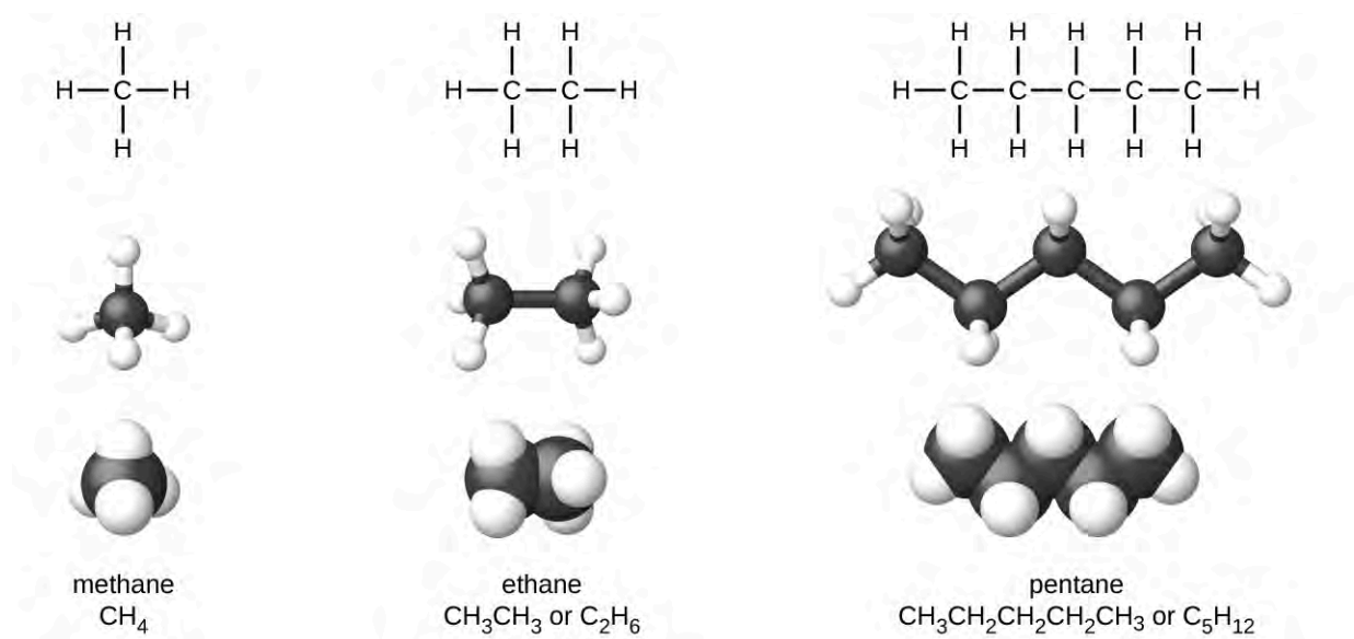
Figure 20.2 Pictured are the Lewis structures, ball-and-stick models, and space-filling models for molecules of methane, ethane, and pentane.
