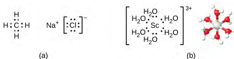
Figure 19.13 (a) Covalent bonds involve the sharing of electrons, and ionic bonds involve the transferring of electrons associated with each bonding atom, as indicated by the colored electrons. (b) However, coordinate covalent bonds involve electrons from a Lewis base being donated to a metal center. The lone pairs from six water molecules form bonds to the scandium ion to form an octahedral complex. (Only the donated pairs are shown.)
