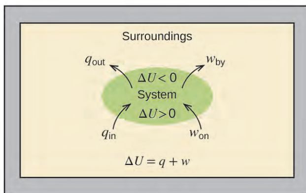
Figure 5.19 The internal energy, U , of a system can be changed by heat flow and work. If heat flows into the system, q_{\text{in}} , or work is done on the system, w_{\text{on}} , its internal energy increases, \Delta U > 0 . If heat flows out of the system, q_{\text{out}} , or work is done by the system, w_{\text{by}} , its internal energy decreases, \Delta U < 0 .
