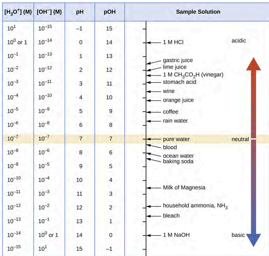
Figure 14.2 The pH and pOH scales represent concentrations of [\text{H}_3\text{O}^+] and \text{OH}^- , respectively. The pH and pOH values of some common substances at standard temperature (25 °C) are shown in this chart.
