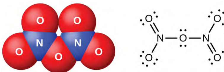
Figure 18.38 This image shows the molecular structure and one resonance structure of a molecule of dinitrogen pentaoxide, N 2 O 5 .
