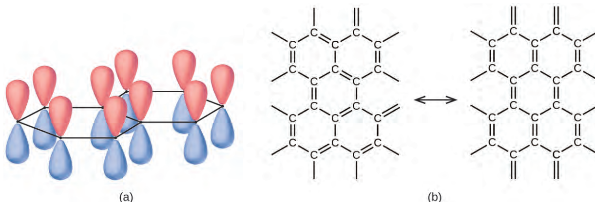
Figure 18.21 (a) Carbon atoms in graphite have unhybridized p orbitals. Each p orbital is perpendicular to the plane of carbon atoms. (b) These are two of the many resonance forms of graphite necessary to describe its electronic structure as a resonance hybrid.
