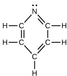
pyridine, trigonal planar, sp^2
