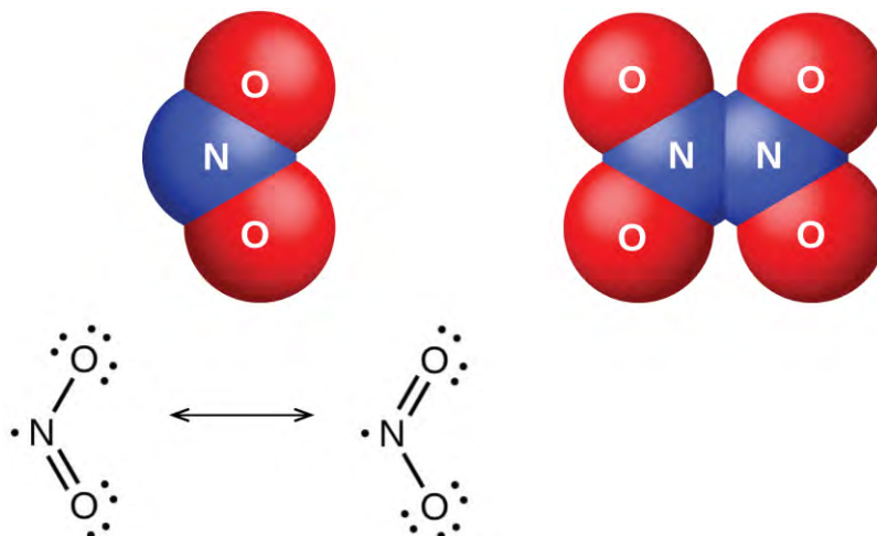
Figure 18.37 The molecular and resonance structures for nitrogen dioxide (NO 2 , left) and dinitrogen tetroxide (N 2 O 4 , right) are shown.
