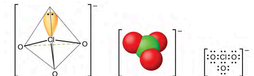
Figure 18.56 Chlorate ions, \text{ClO}_3^- , are produced when halic acids react with bases.
