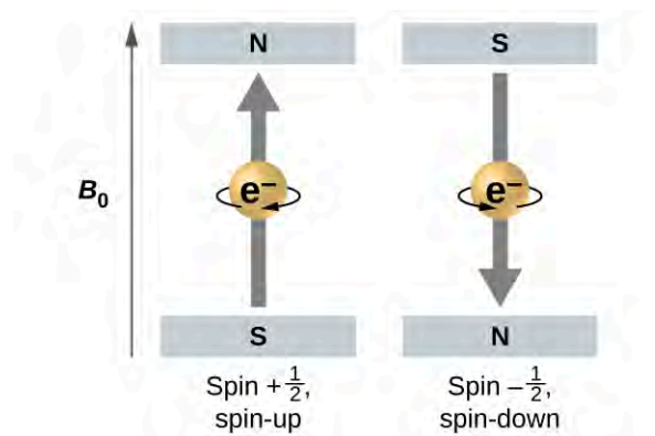
Figure 6.24 Electrons with spin values \pm\frac{1}{2} in an external magnetic field.
