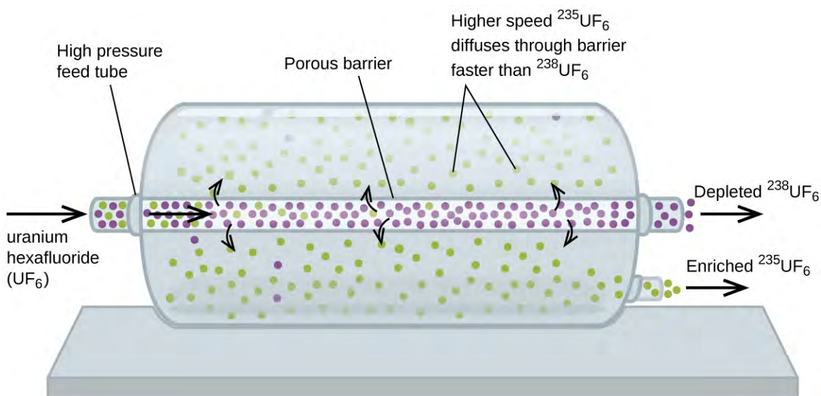
Figure 9.30 In a diffuser, gaseous UF 6 is pumped through a porous barrier, which partially separates 235 UF 6 from 238 UF 6 . The UF 6 must pass through many large diffuser units to achieve sufficient enrichment in 235 U.
