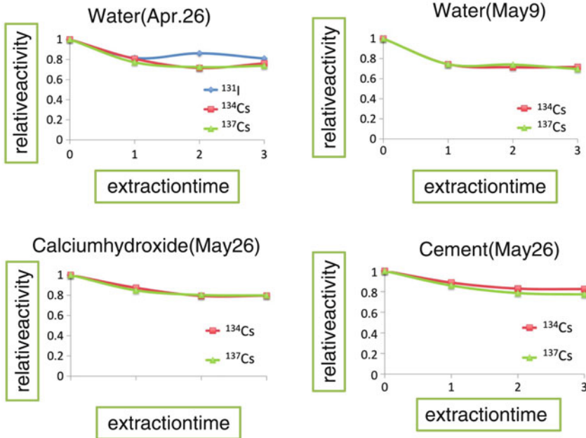
Fig. 1.4 Extraction of radioactive nuclides from paddy soil for a rice plant. Soil was washed under different treatments to find out in which condition the radioactivity can be removed from the soil
