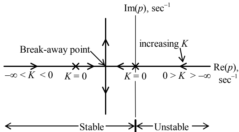
Figure 16-6 Loci of roots of p^2 + 2Cp + K = 0 as K varies from -\infty to greater than C^2 , with C > 0 held constant
