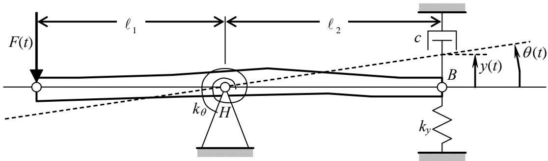
Figure 11-3 Example 11-1: damped, spring-supported, hinged rigid bar
