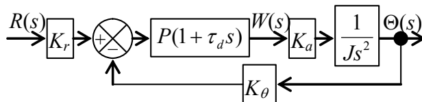
Figure 15-8 Ideal proportional-derivative (PD) control of rotor position
