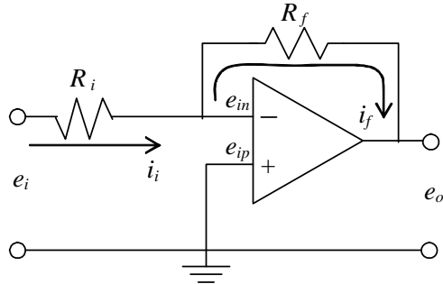
Figure 5-8 Inverting amplifier
