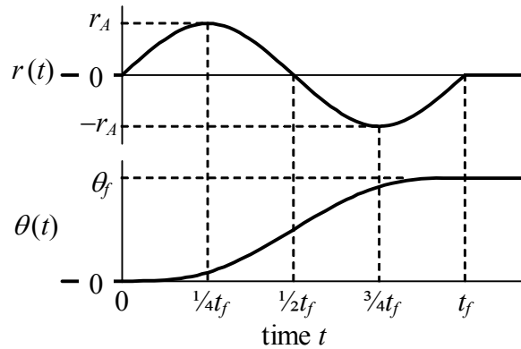
Figure 14-4 Example operator setting and resulting pitch maneuver for re-entry capsule
