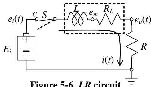
Figure 5-6 LR circuit
