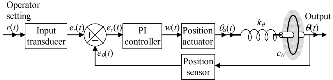
Figure 15-4 Functional diagram of a system for controlling the position of a spring-connected rotor in a viscous liquid, based on proportional-integral control
