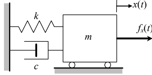
Figure 9-1 Mass-dashpot-spring system
