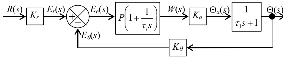
Figure 15-5 Laplace block diagram of a system for controlling the position of a spring-connected rotor in a viscous liquid, based on proportional-integral control
