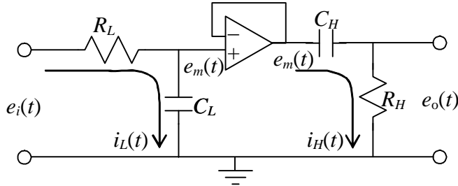
Figure 5-10 RC band-pass filter
