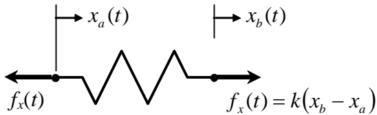
Figure 3-7 Ideal linear spring with stiffness constant k
