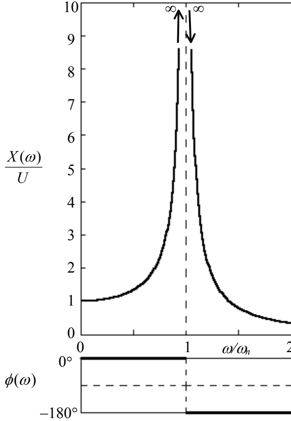
Figure 10-1 Frequency response function of an undamped 2 nd order system
