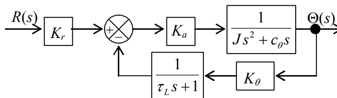
Figure 16-3 Laplace block diagram of position-feedback control system with low-pass filtering
