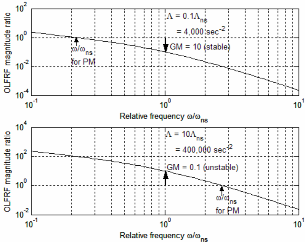
Figure 17-3 Magnitude ratios, Eq. (17-5) for \Lambda = 4,000 and 400,000 \text{ sec}^{-2}
