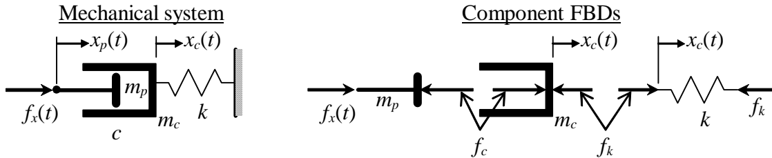
Figure 3-11 Example series mass-dashpot-spring
