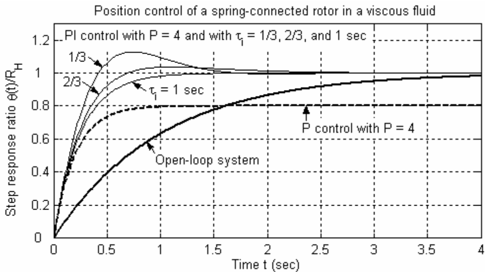
Figure 15-6 Step responses for no control (open-loop), proportional (P) control, and proportional-integral (PI) control
