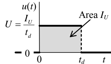
Figure 8-2 Flat impulse
