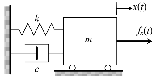
Figure 7-1 Mass-damper-spring system
