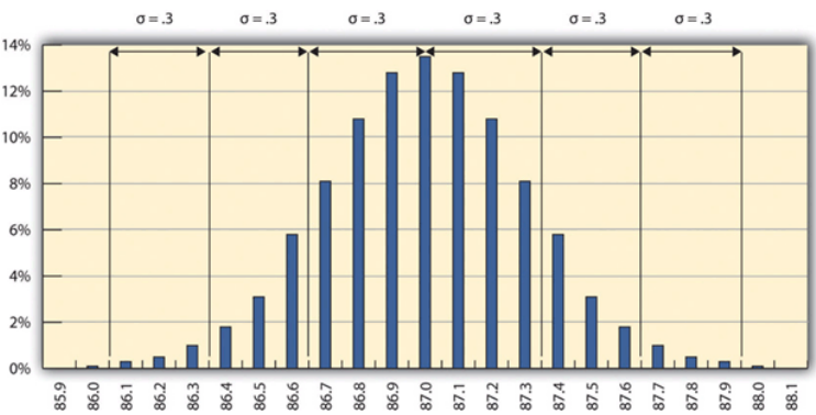
Figure 10.3 The 68-95-99.7 Rule
