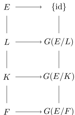
Figure 23.23: Subgroups of G(E/F) and subfields of E
