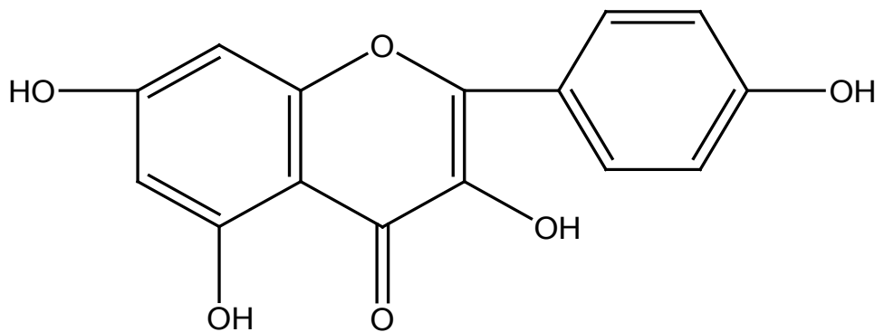
Figure 7: Kaempferol.
