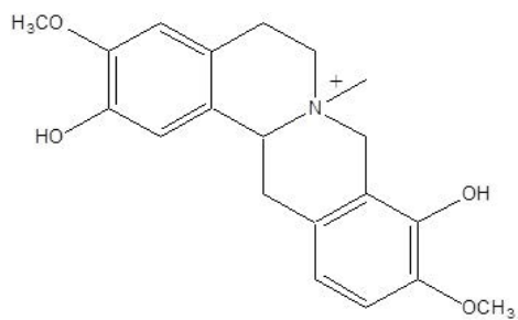
Figure 6: Cissamine.
