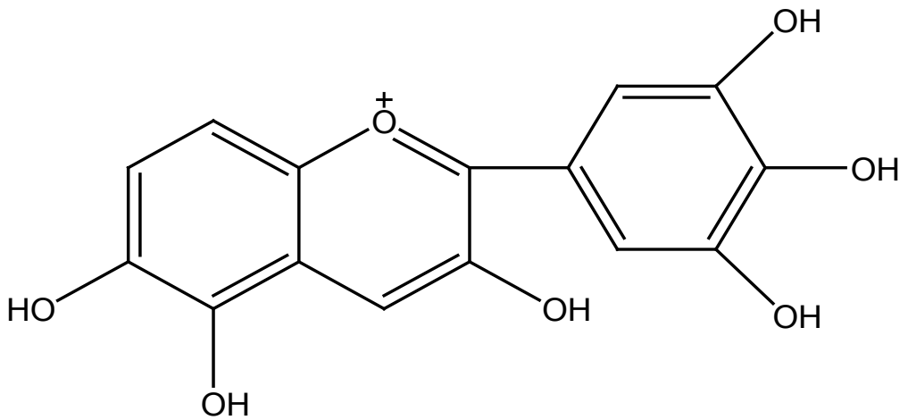
Figure 6: Delphinidin.
