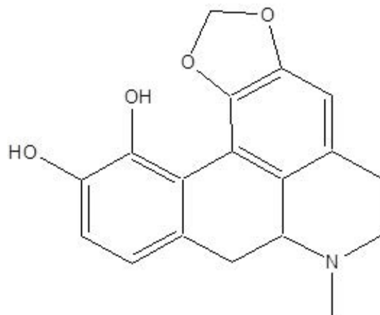
Figure 11: Bulbocarpine.
