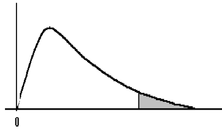
The \chi^2 distribution
