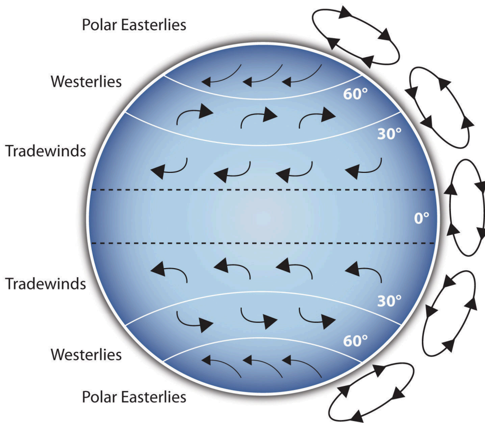
Figure 15.1 Coriolis Effect
