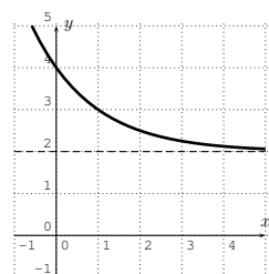
horizontal asymptote
