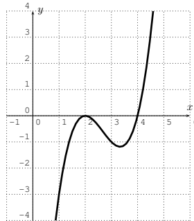
2 roots, 2 extrema
