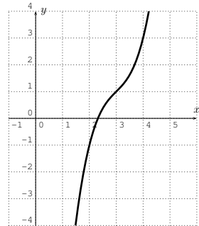
1 root, 0 extrema
