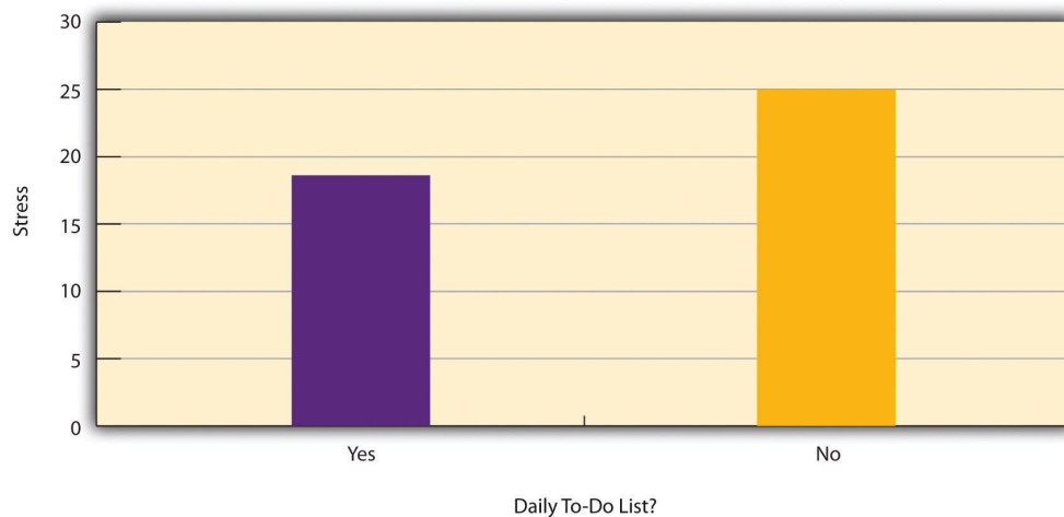
Figure 7.2 Results of a Hypothetical Study on Whether People Who Make Daily To-Do Lists Experience Less Stress Than People Who Do Not Make Such Lists
