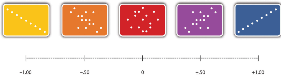
Figure 2.4 Range of Pearson’s r , From -1.00 (Strongest Possible Negative Relationship), Through 0 (No Relationship), to +1.00 (Strongest Possible Positive Relationship)
